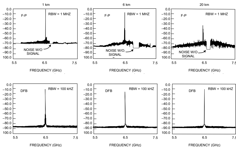
Figure 20. Comparative Noise Performance for DFB and F-P Lasers
